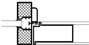
DEKO FG fully glazed partition
